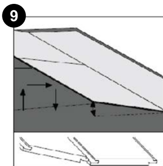
Fixing edge trim to wall
