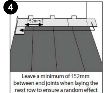
Use of offcut from previous row (optimal)
