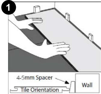
Laying first plank in corner of room with tongue side facing wall using 5mm spaces
