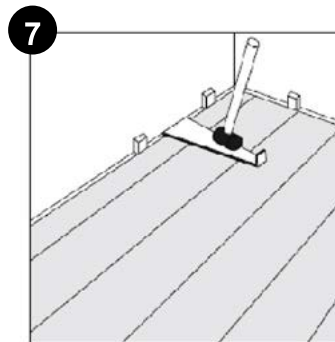
Pull bar and rubber mallet can be used for final row of planks, ensuring a 5mm expansion gap
