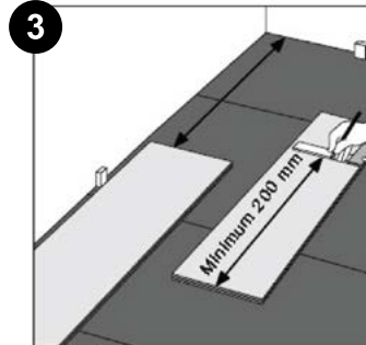
Cutting and fitting of final plank in first row
