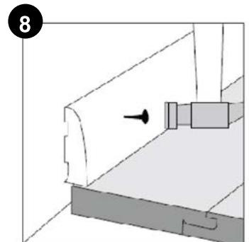
Refitting of skirting board with hidden 5 mm expansion gap
